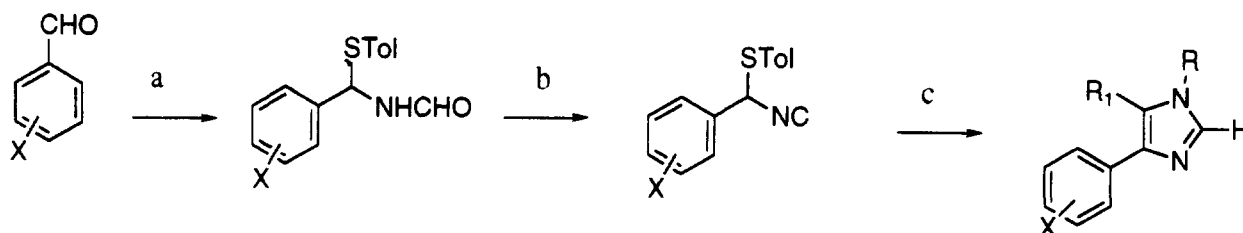
Scheme 2. Synthesis of N-1-alkyl-4,5-diarylpyridines: (a) TolSH, NCONH 2 ; (b) POCl 3 ; (c) R 1 =NR, TBD.
