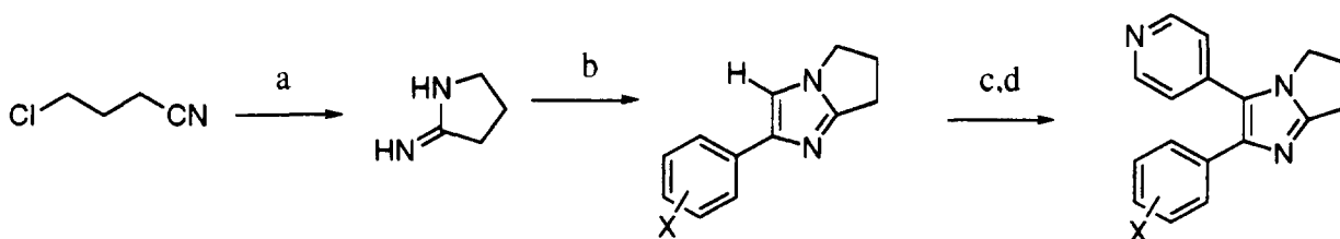
Scheme 3. Synthesis of 2,3-diarylpyrroloimidazoles: (a) NH 3 , NaOCH 3 ; (b) X-PhC(O)CH 2 Cl; (c) C 5 H 5 N, EtOC(O)Cl; (d) tert -BuOK, tert -BuOH.
